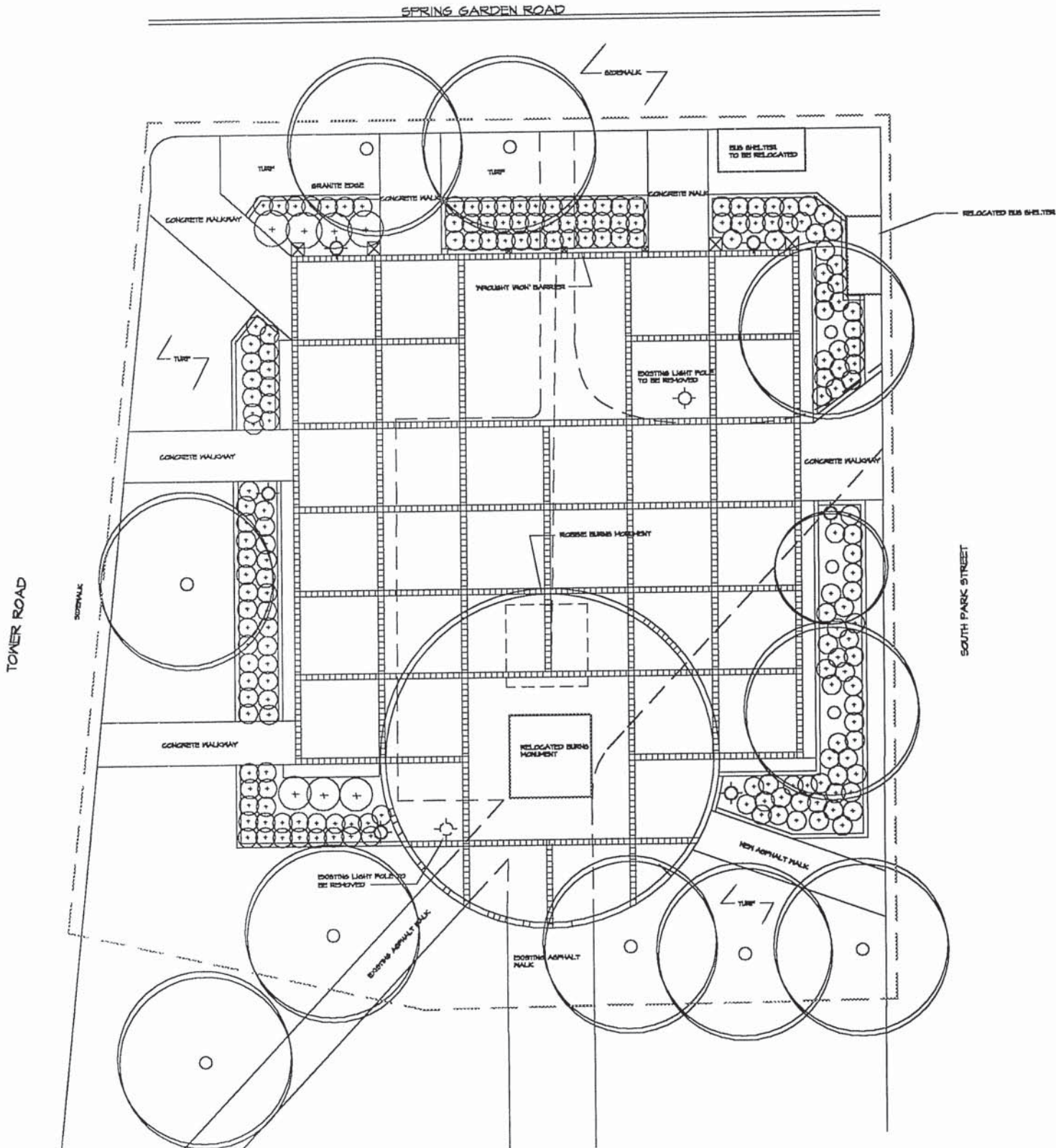
PROPOSED IMPROVEMENTS - VICTORIA PARK L-1 1" = 10'
