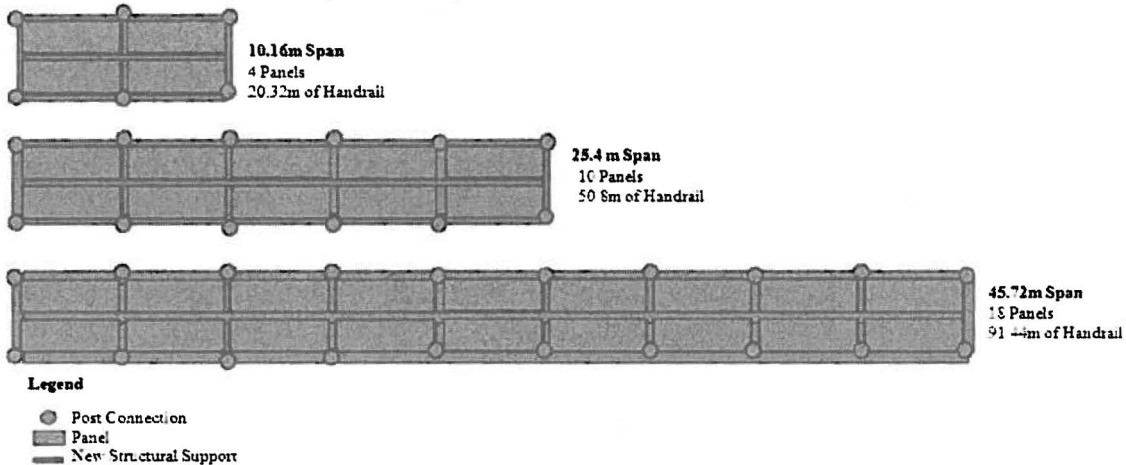
Figure 2: Required Material by Bridge Length – Alignment A
