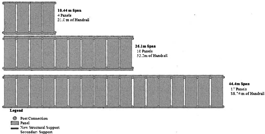
Figure 3: Required Material by Bridge Length – Alignment B
