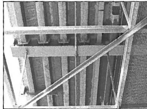
Deck panels as seen from below.
