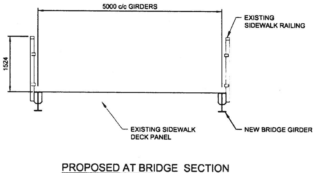
Figure 4: Proposed Bridge Section
